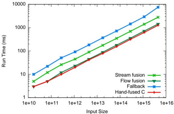
QuickHull benchmark
