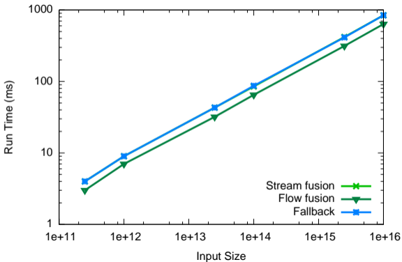
MapMap benchmark
