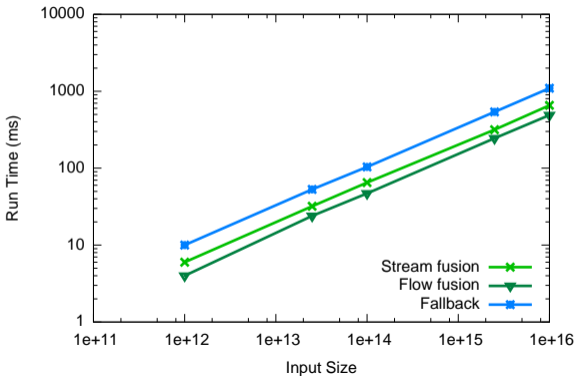
Dot Product benchmark
